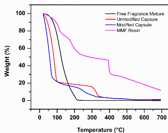
Figure 4. TGA diagrams.
