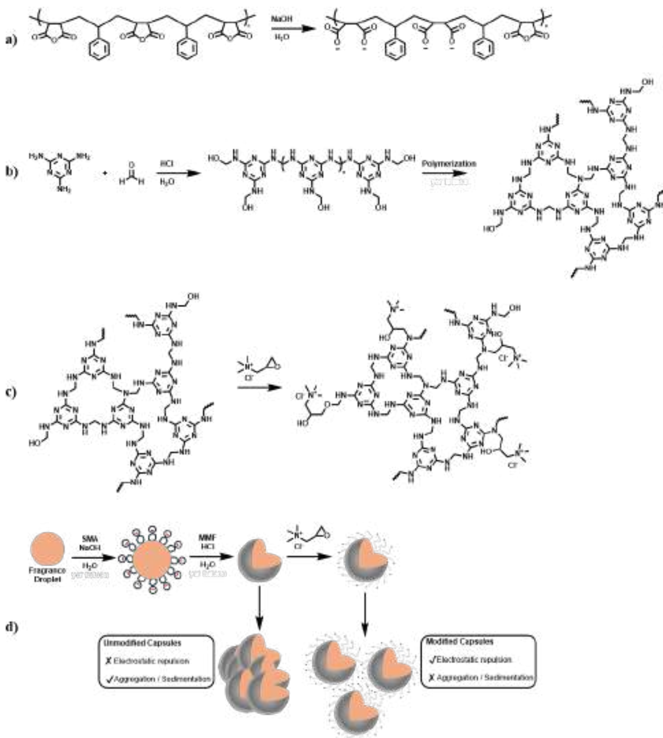
Scheme 1. Schematic overview of the structural representation of styrene-maleic anhydride copolymer before and after hydrolysis (a), in situ polymerization of MMF (b), post-curing cationic surface functionalization of the microcapsules with glycidyl trimethylammonium chloride (c), proposed influence of surface functionalization on dispersion behaviour (d).
