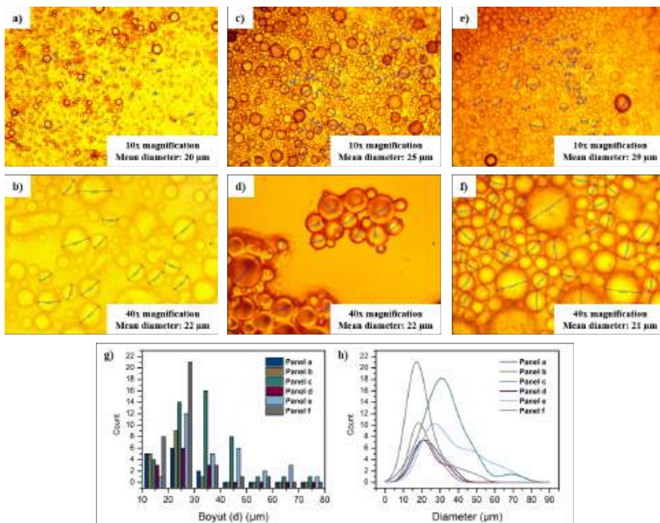
Figure 2. Optical microscopy images of fragrance-loaded microcapsules (Pink Capsule ENC Last) recorded after 30 min of reaction (a) , (b) , after 2 h of curing and before the addition of glycidyl trimethylammonium chloride (c) , (d) , after glycidyl trimethylammonium chloride addition and cooling to room temperature (e) , (f) , and particle-size histograms and distribution curve (g) , (h) . (Mean diameters were calculated from the particles measured in the corresponding images, smoothed curve was obtained with the Gaussian Kernel Method and derived from the same datasets).
