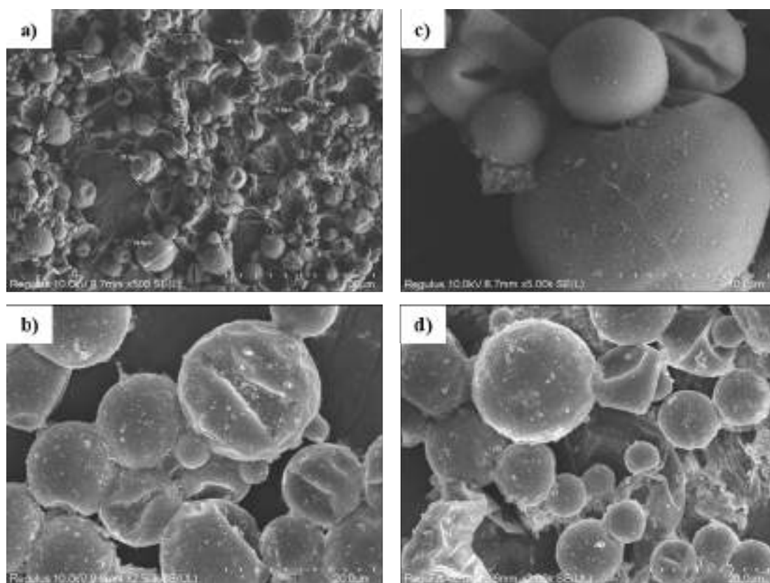
Figure 3. SEM images of fragrance-loaded (Pink Capsule ENC Last) microcapsules obtained at 500× magnification (a), 2500× magnification (b), 5000× magnification (c), 2000× magnification before treatment (d).
